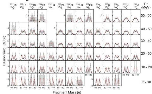
Fig.1 FFMD obtained in the MNT channels in ^{18}\text{O} + ^{232}\text{Th} . The curves are the Langein model calculation [2].
